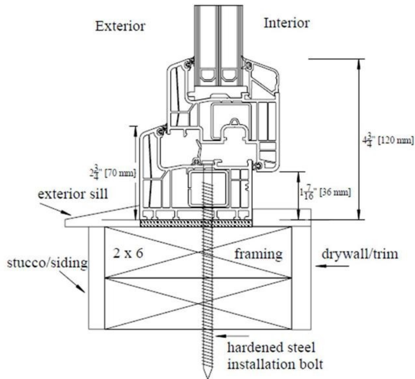
Typical installation of a tilt & turn window into wood framing
